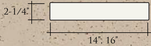
SST-404 PROFILE (SIDE VIEW)
